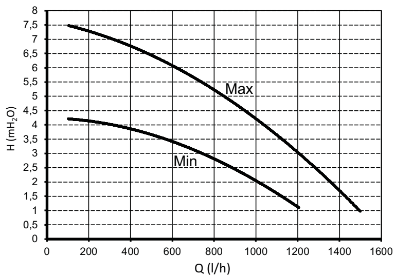
STAR CONDENS NEXT 1.32
