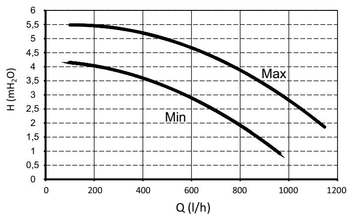
STAR CONDENS NEXT 1.32
